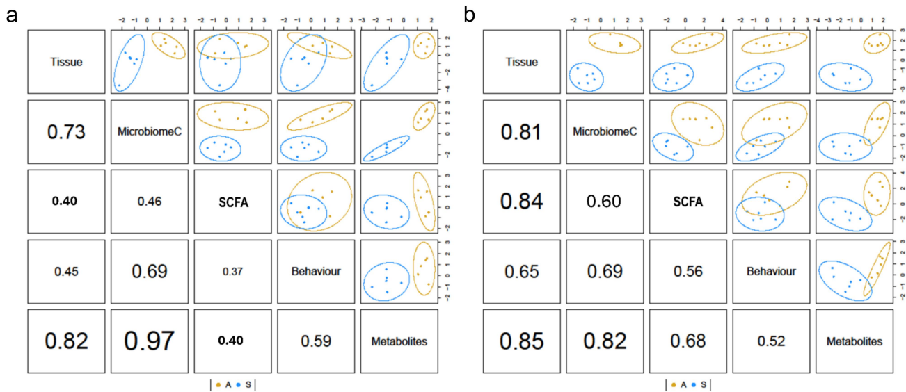
Figure 8. Correlative analysis supports the involvement of the microbiota-gut-brain axis in ASD-like phenotype. Representation of correlation values and 2D discrimination plots of integrative analysis after dimensionality reduction technique of the data in (a) BL/6 and (b) Balb/c transplanted mice. Components are formed so that they maximize the correlation between the different datatypes as well as the phenotype. The data block named as tissue includes all molecular outcomes measured in gut, spleen and brain representing host's biological responses.
